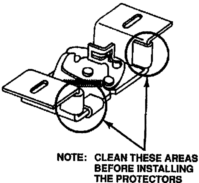
Fig. 2: Installing Protectors
