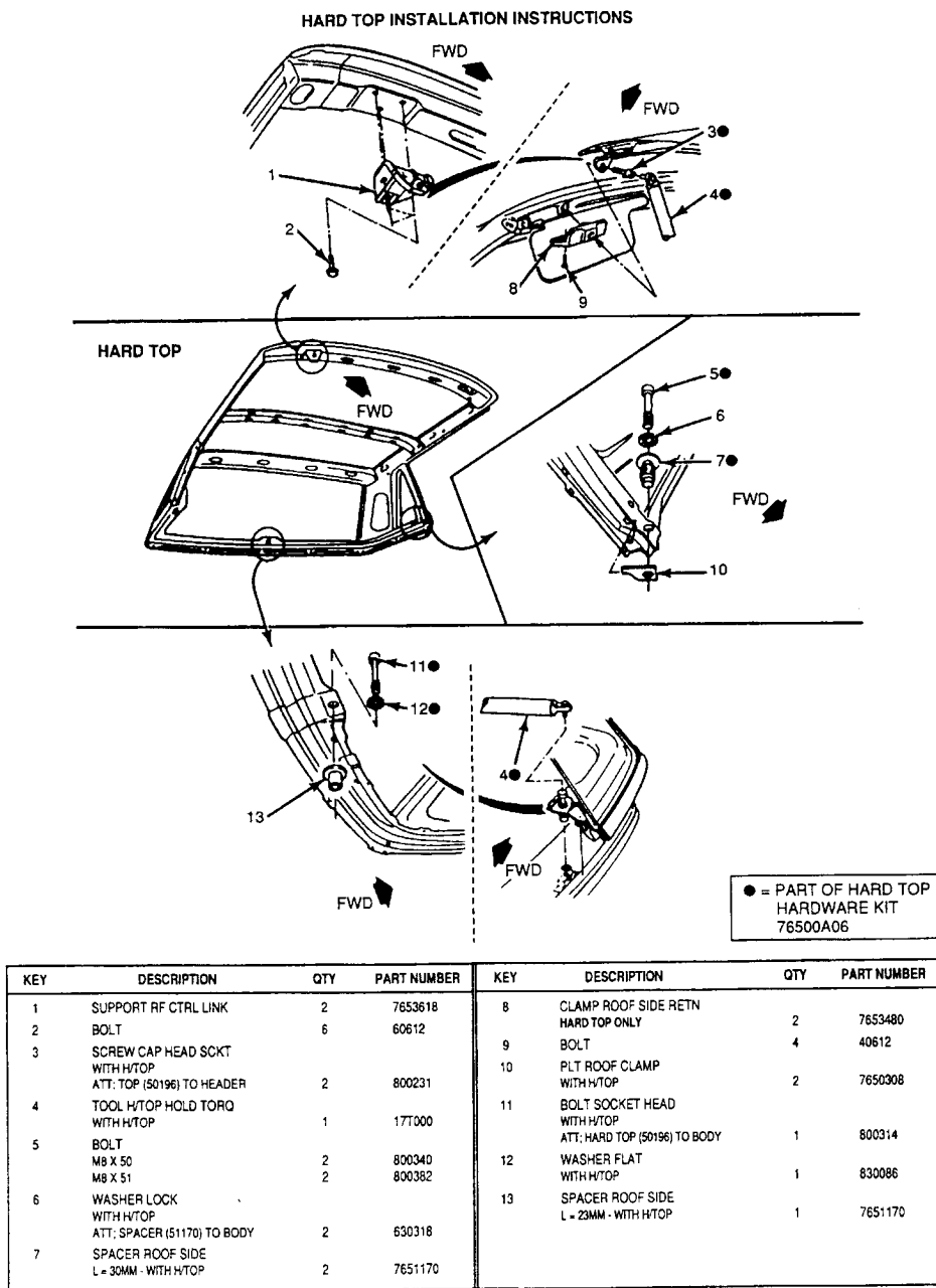
Fig. 3: Hard Top - Installation Instruction
